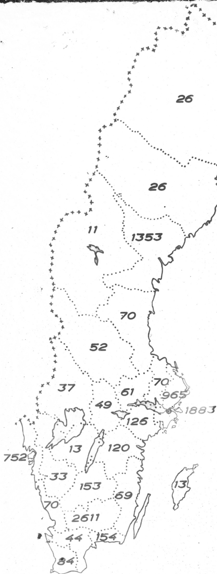
Fig. 4. Number of cases of S. typhimurium from June 9th until Dec. 28th within different provinces of Sweden.
